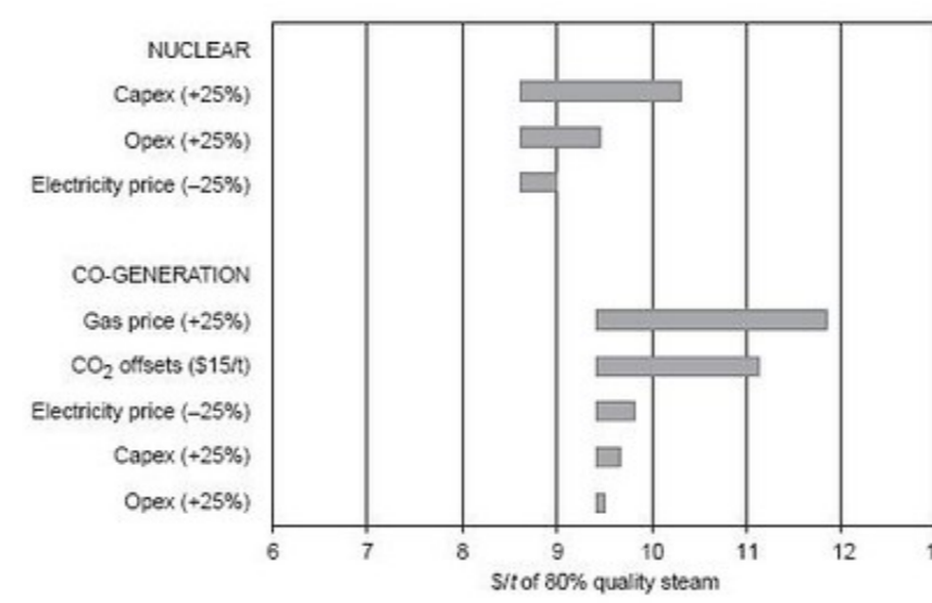
Fig. 3. Steam supply cost sensitivities
